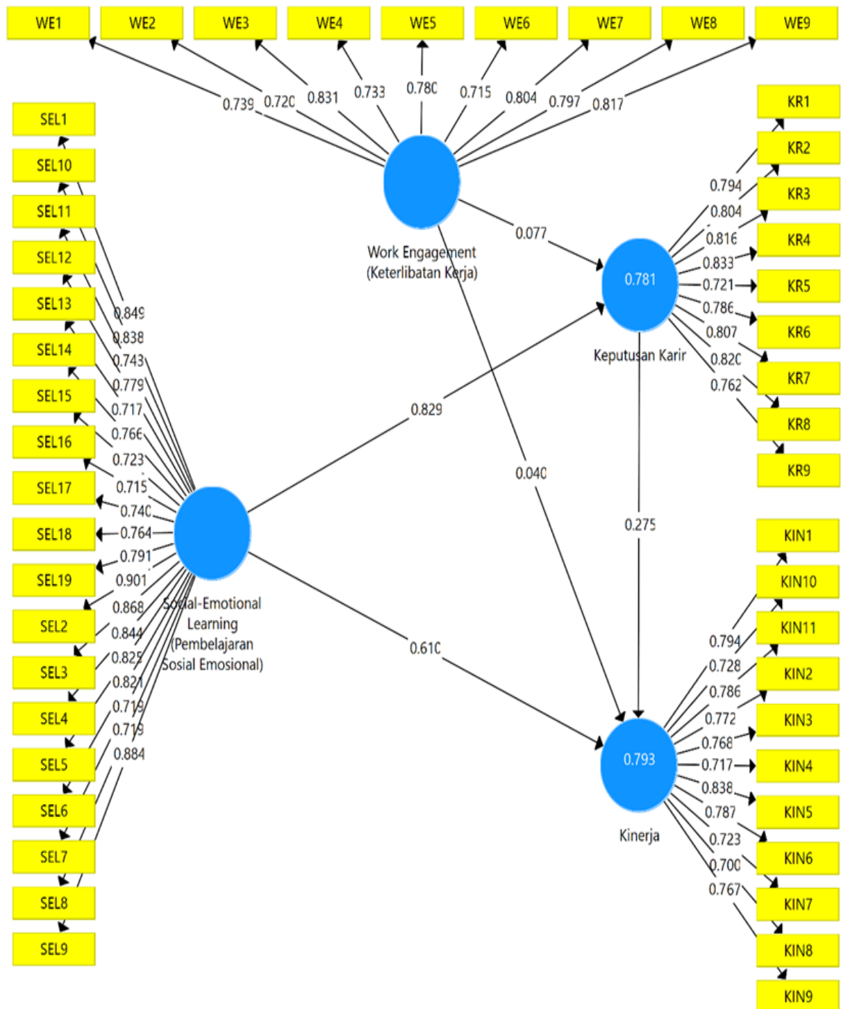
Figure 2. PLS (Loading Factor Manifest) algorithm Source: Processing results SmartPLS v.3.2.9 (2024)
