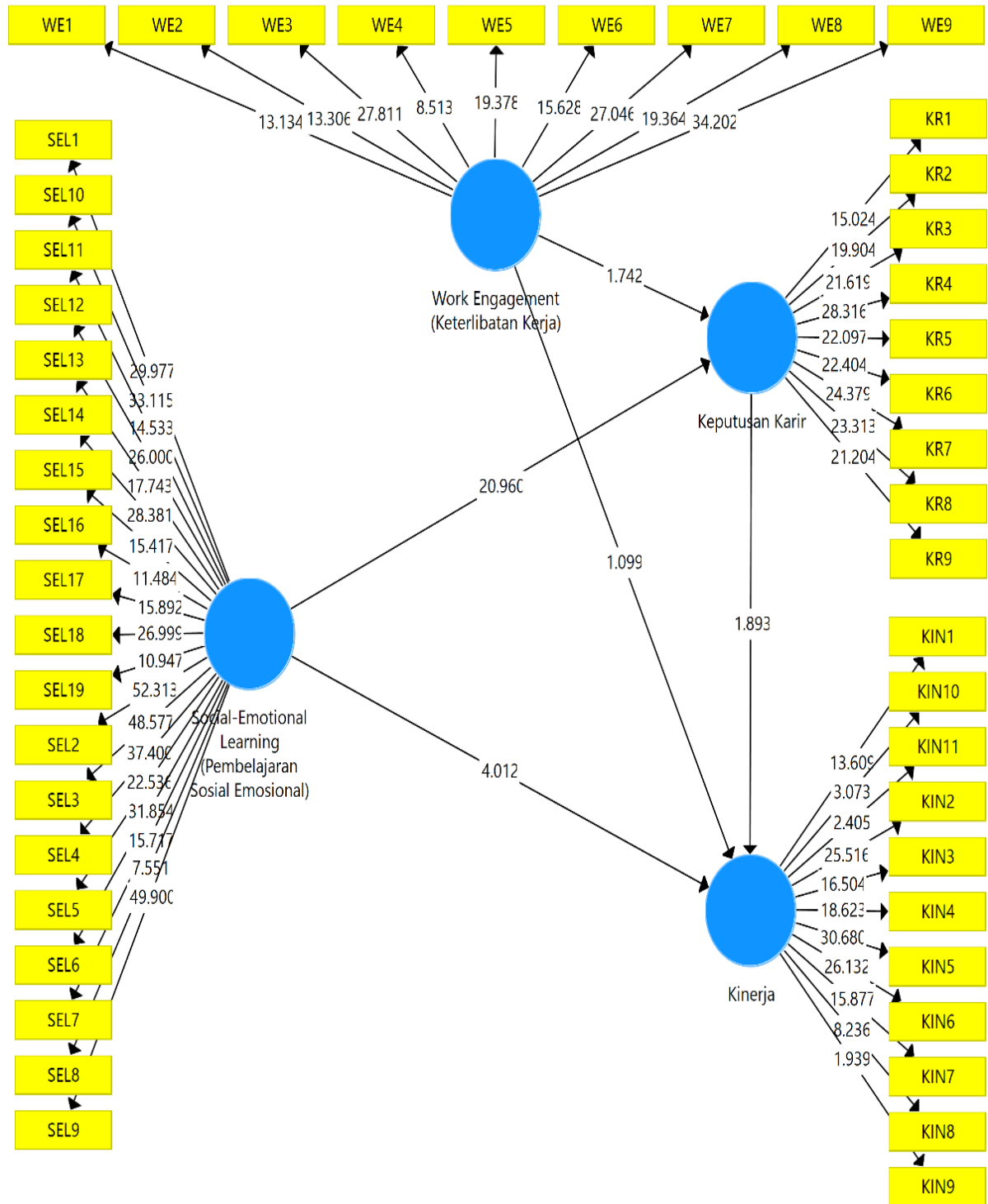
Figure 3. Significance Test of Bootstrapping Model Source: Data processed by SmartPLS v.3.2.9 (2024)
