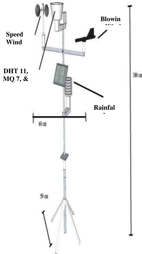
Figure 2. Prototype Design
