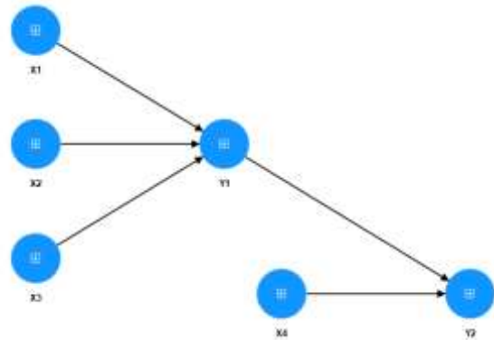
Figure 3. UTAUT model
