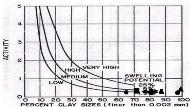
Figure 4. Graph of Activity Analysis Results with Variations in SBE Content and Non Curing [9]
