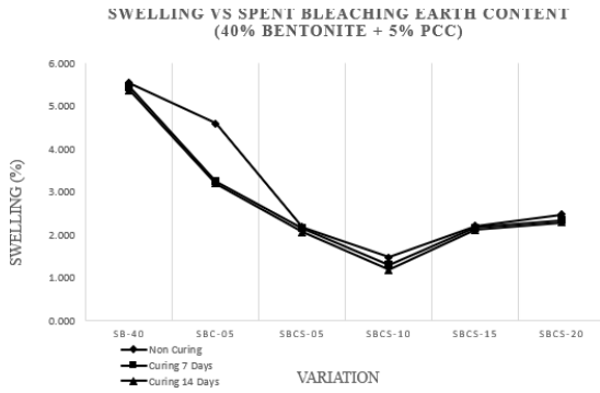
Figure 7. Graph of Swelling Results with Variations in SBE Content and Curing Time
